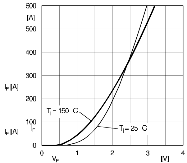
Fig. 10: Typ. CAL diode forward charact., incl. R_{CC'+EE'}
